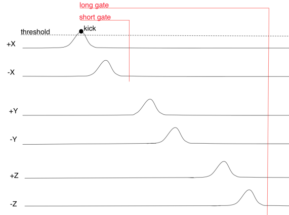
Figure 3. Kick detection.
