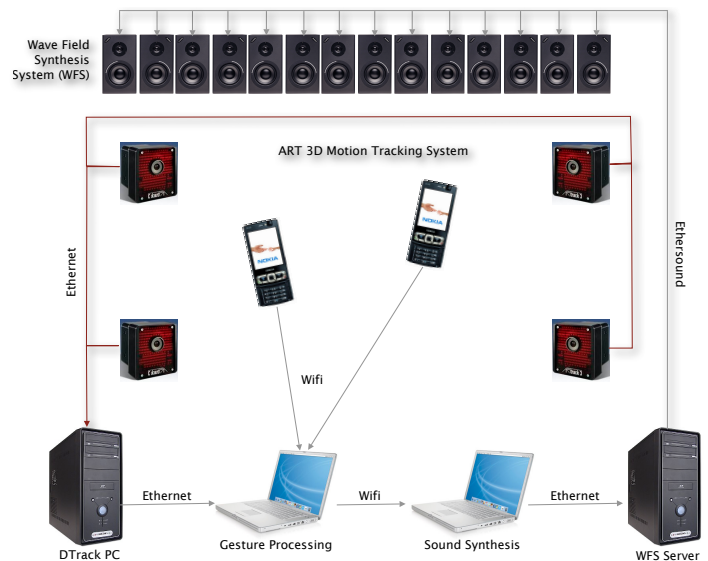
Figure 1. Diagram of the installation hardware setup with the communication protocols between components.
