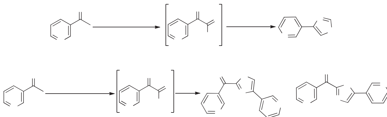
Scheme 1. The cascade DMSO-HBr oxidation and Debus-Radziszewski condensation procedure.
