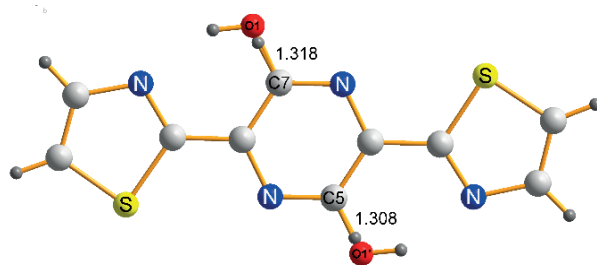
Figure 3. The X-ray molecular structure of 3p .
