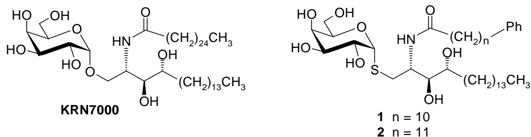
Figure 1. Structures of KRN7000 and target molecules 1 and 2 .
