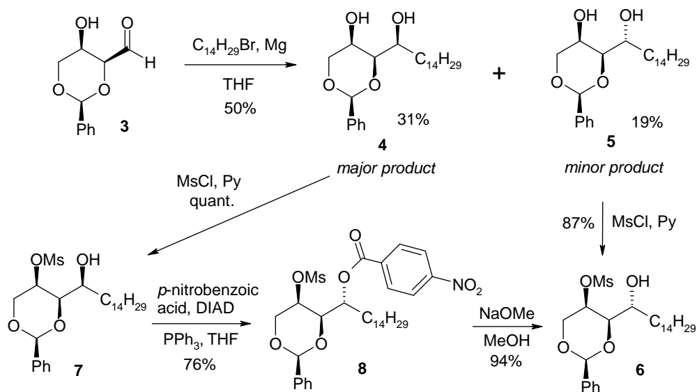
Scheme 1. Synthesis of intermediate 6 .
